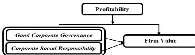
Figure 1. Framework
