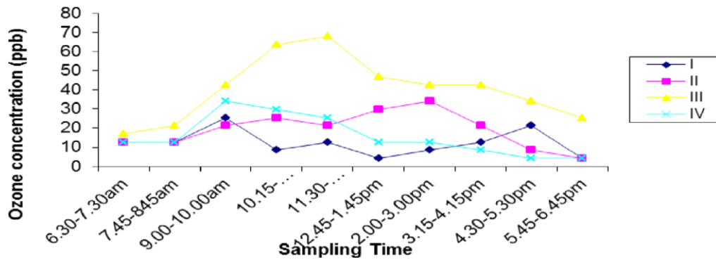
Figure 12: Time Variation of Daily Average Concentration of Ozone in Ilorin Town during Wet Season Thus NO x dominated the polluted air shed in Ilorin in the morning to mid-afternoon, and by O 3 in the late afternoon. The atmospheric turbidity during the Harmattan season is generally known to be high, inhibiting optimal surface penetration of solar radiation. As a result, the rates of atmospheric photochemical kinetic processes are expected to be low. This implies that O 3 production currently recorded may be lower than the atmospheric concentrations outside the peak Harmattan season. To enable the quantitative evaluation of the potential role played by Harmattan aerosol in the O 3 photochemical production process, the typical seasonal variability of solar radiation level during an annual cycle in Ilorin is presented in Figure 13.
