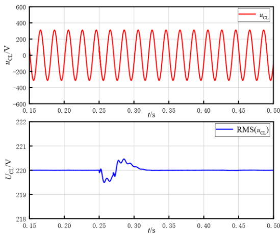
Figure 11: Changes in u_{CL} when switching non-critical loads.
