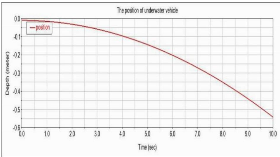
Figure 14: The change of the position of the center of mass in the first 10 seconds when eight pendulums flap simultaneously.
