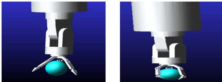
Figure 17: Grasping process.
