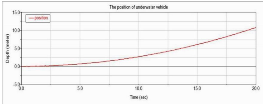
Figure 7: The relationship between the position of AUV's center of mass and time when AUV descent.
