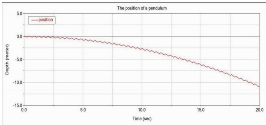
Figure 6: The relationship between pendulum's position and time when AUV ascent.
