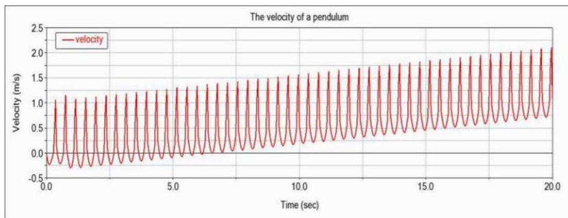
Figure 8: The relationship between pendulum's velocity and time when AUV descent.
