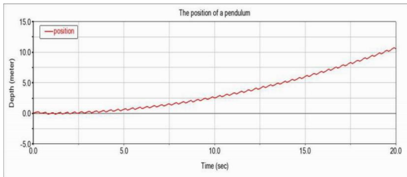
Figure 9: The relationship between pendulum's position and time when AUV descent.
