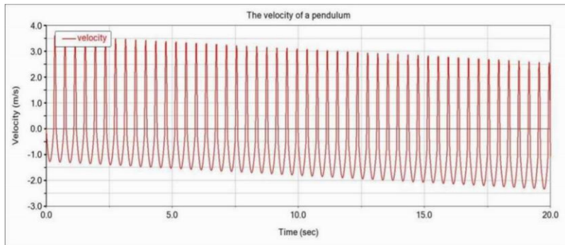
Figure 5: The relationship between pendulum's velocity and time when AUV ascent.
